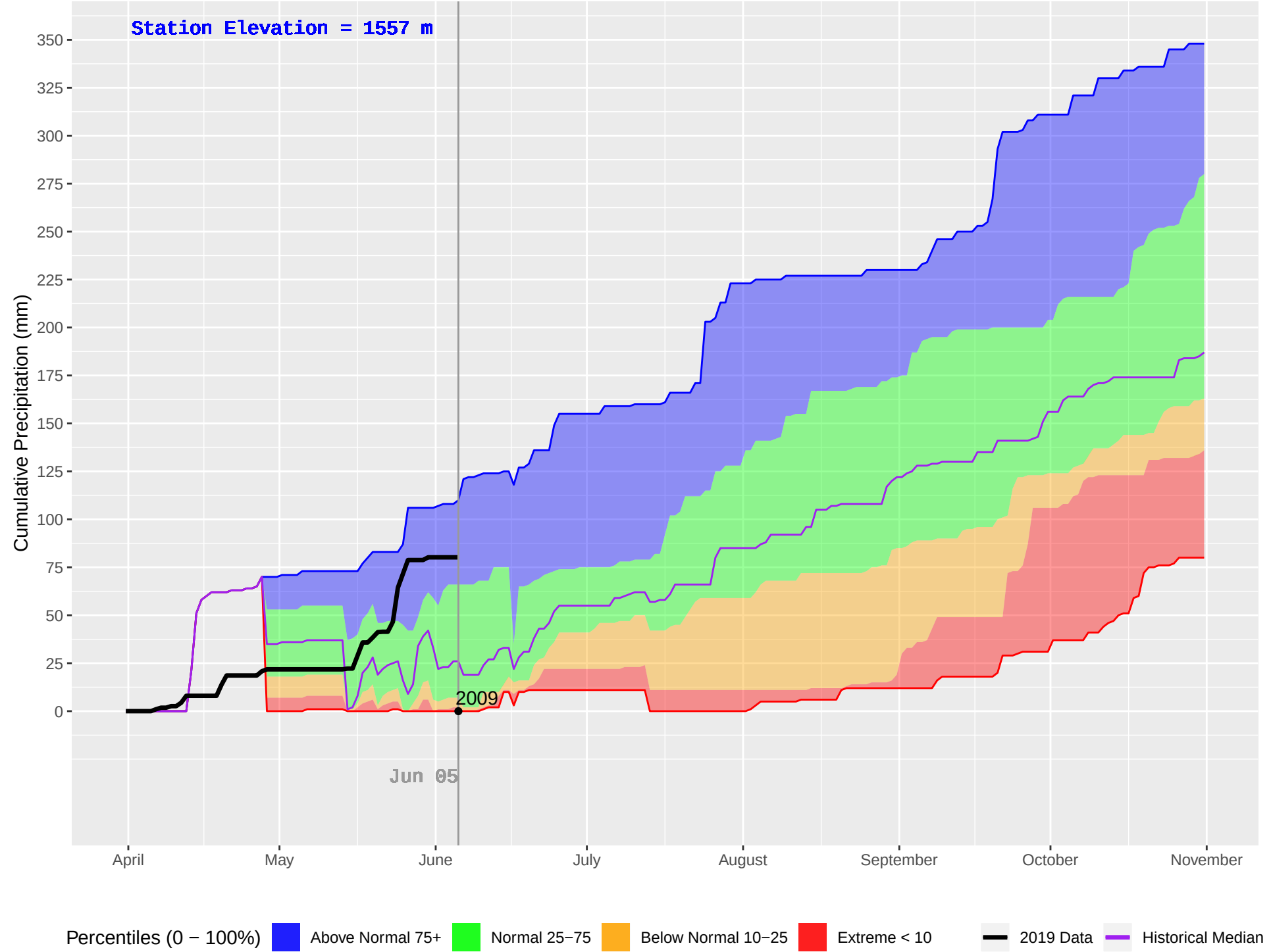
SKOONKA (1024) : Historical (2008–2018), Current (2019) Daily Cumulative Precipitation
