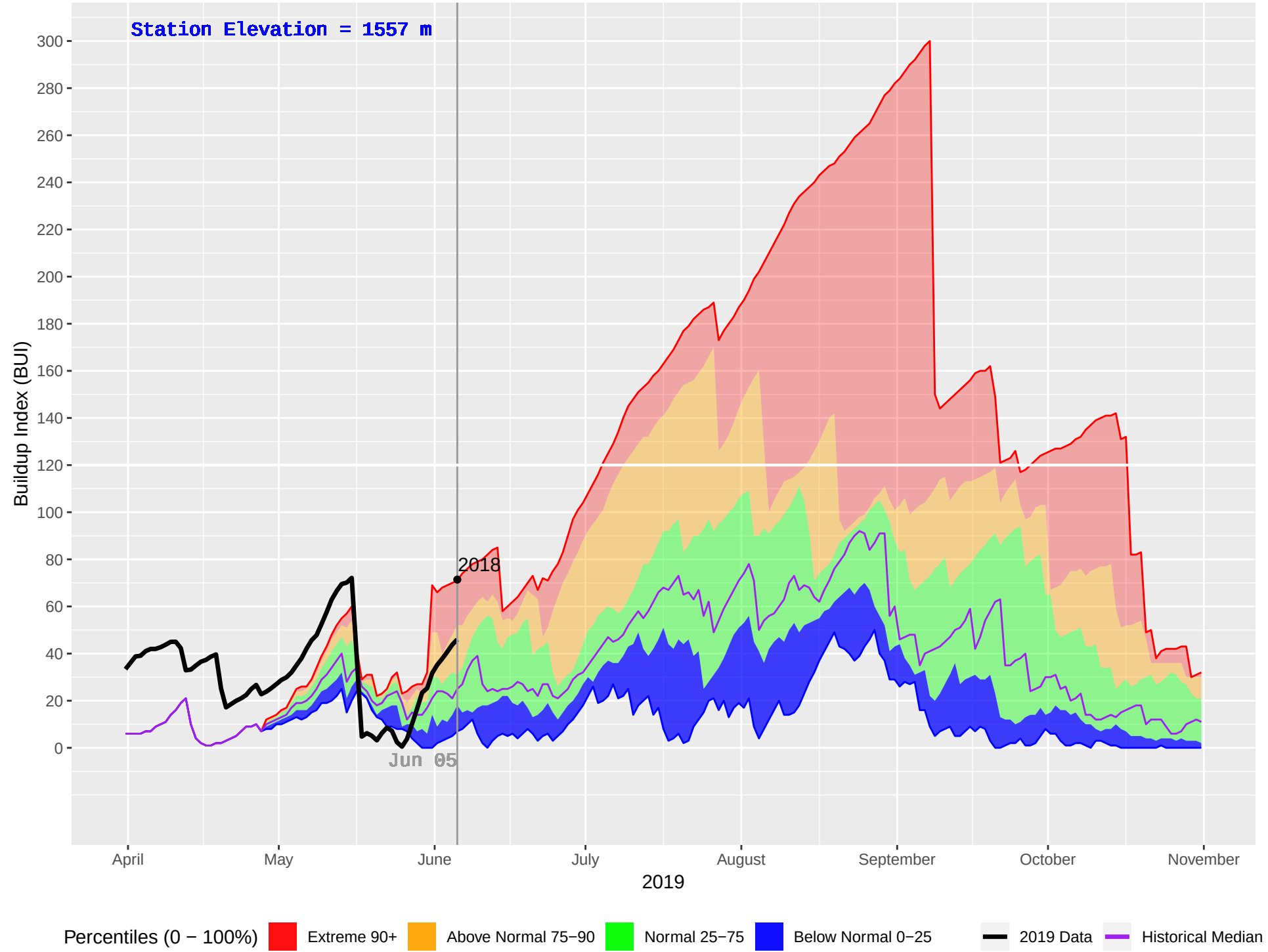
SKOONKA (1024) : Historical (2008–2018), Current (2019) Daily Buildup Index (BUI)
