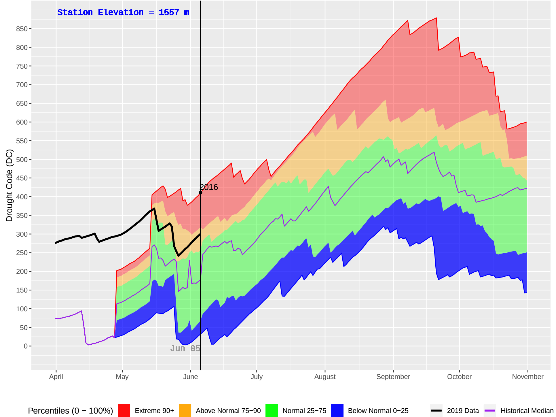
SKOONKA (1024) : Historical (2008–2018) and Current (2019) Daily Drought Code (DC)
