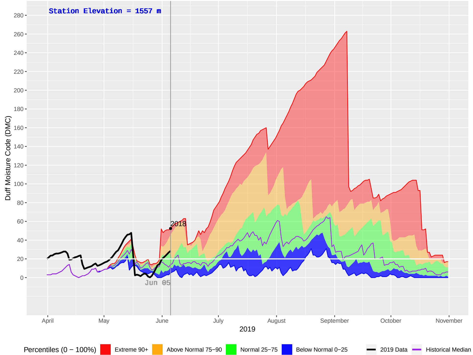
SKOONKA (1024) : Historical (2008–2018), Current (2019) Daily Duff Moisture Code (DMC)
