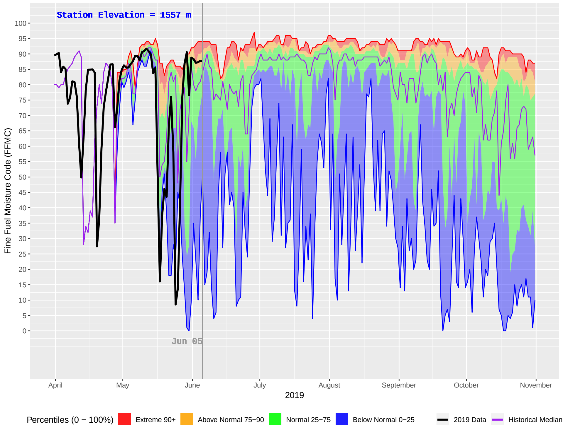
SKOONKA (1024) : Historical (2008–2018) and Current (2019) Daily Fine Fuel Moisture Code (FFMC)
