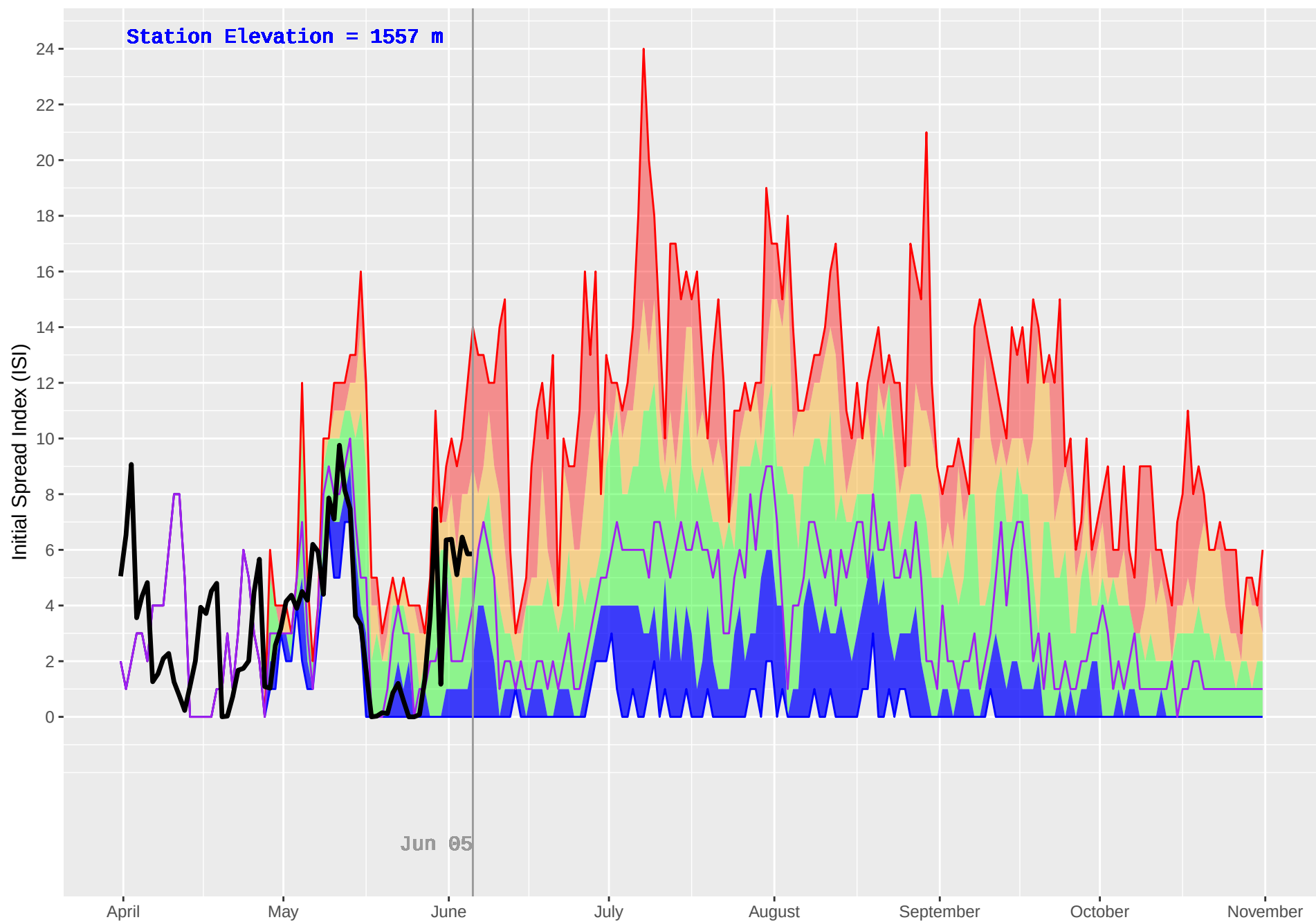
SKOONKA (1024) : Historical (2008–2018) and Current (2019) Daily Initial Spread Index (ISI)
