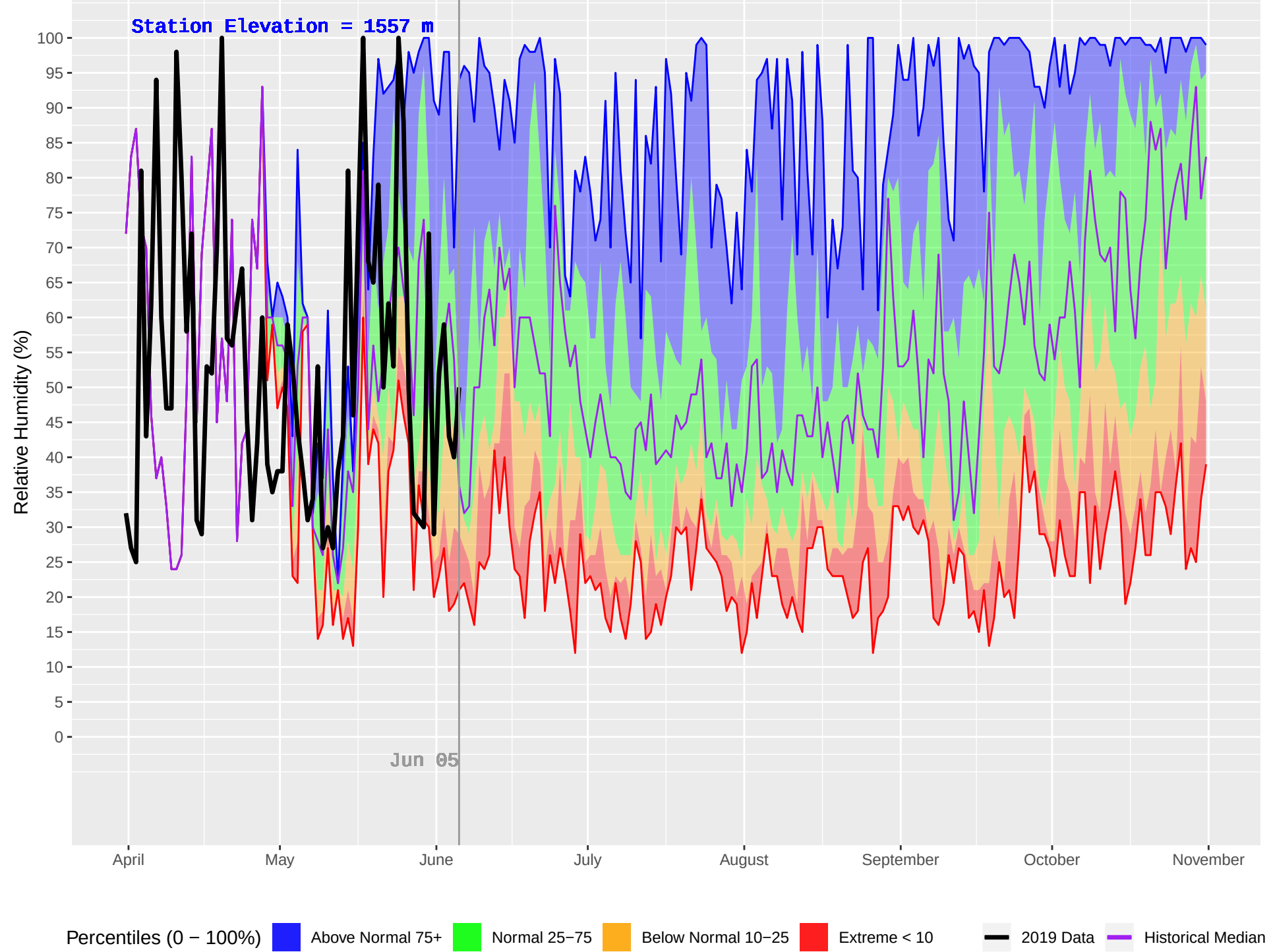
SKOONKA (1024) : Historical (2008–2018) and Current (2019) Daily Relative Humidity
